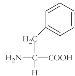
Phenylalanine
